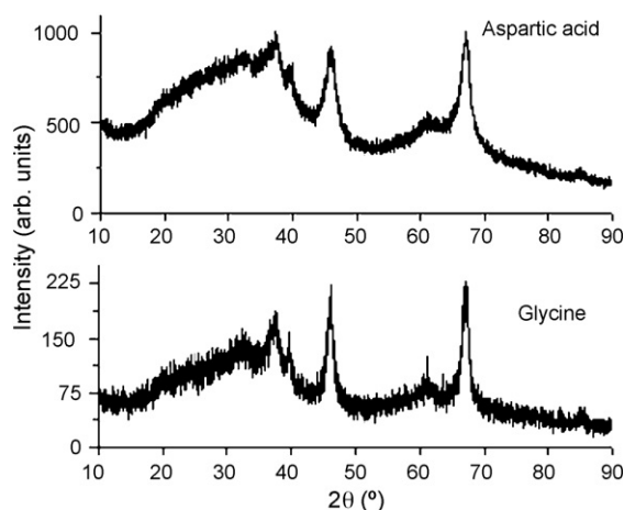
Fig. 3. Comparison between XRD patterns of \text{Al}_2\text{O}_3 nanopowders synthesized by stoichiometric nitrate–aspartic acid and nitrate–glycine routes calcined at 800 °C.
