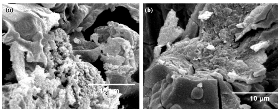
Fig. 5. SEM micrographs of \text{Al}_2\text{O}_3 nanopowders exhibiting the metastable \gamma phase. (a) Non-stoichiometric nitrate–aspartic acid route calcined at 900 °C. (b) Stoichiometric nitrate–aspartic acid route calcined at 850 °C.
