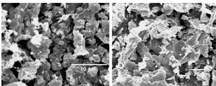
Fig. 6. SEM micrographs of \text{Al}_2\text{O}_3 nanopowders exhibiting the \alpha phase. (a) Non-stoichiometric nitrate–glycine route calcined at 1200 °C. (b) Non-stoichiometric nitrate–aspartic acid route calcined at 1200 °C.
