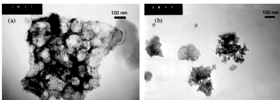
Fig. 7. TEM micrographs showing the typical morphology of \text{Al}_2\text{O}_3 nanopowders exhibiting the metastable \gamma phase. (a) Stoichiometric nitrate–aspartic acid route calcined at 850 °C. (b) Stoichiometric nitrate–glycine acid route calcined at 800 °C.
